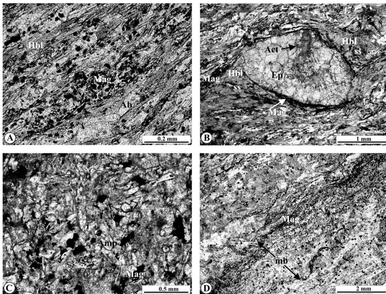
Fig. 2. A – magnetite aggregates parallel to foliation defined by laths of amphibole and plagioclase in streaky amphibolite ; B – ellipsoidal nodule composed of epidote crystals in streaky amphibolite ; in the central part of nodule radial actinolite aggregates occur; cone-shaped strain shadows (ss) adjacent to nodule are filled with bluish-green hornblende; C – mineral framework of massive amphibolite : cloudy albite-epidote aggregate with randomly arranged amphibole laths and magnetite crystals; D – thin, cord-like magnetite aggregates embedded in mylonite zone (mb) parallel to the foliation A-D, plane-polarized light. Hbl – hornblende, Mag – magnetite, Ab – albite, Act – actinolite, Amp – amphibole, Ep – epidote
